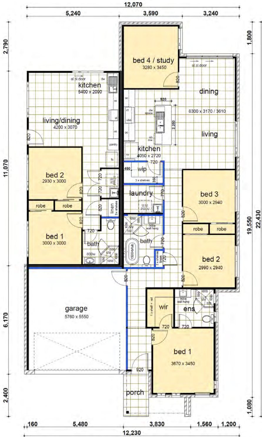
floor plan
