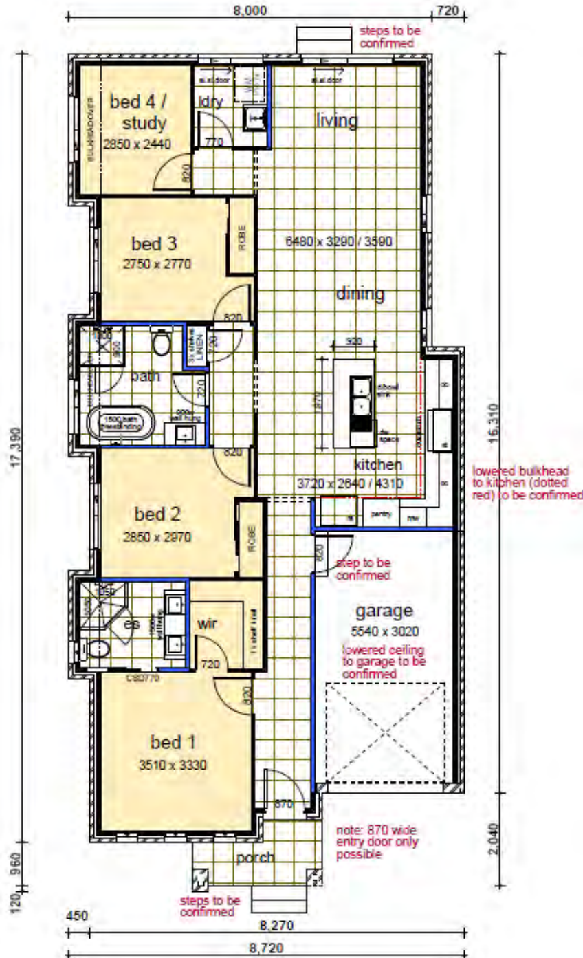
FLOOR PLAN
