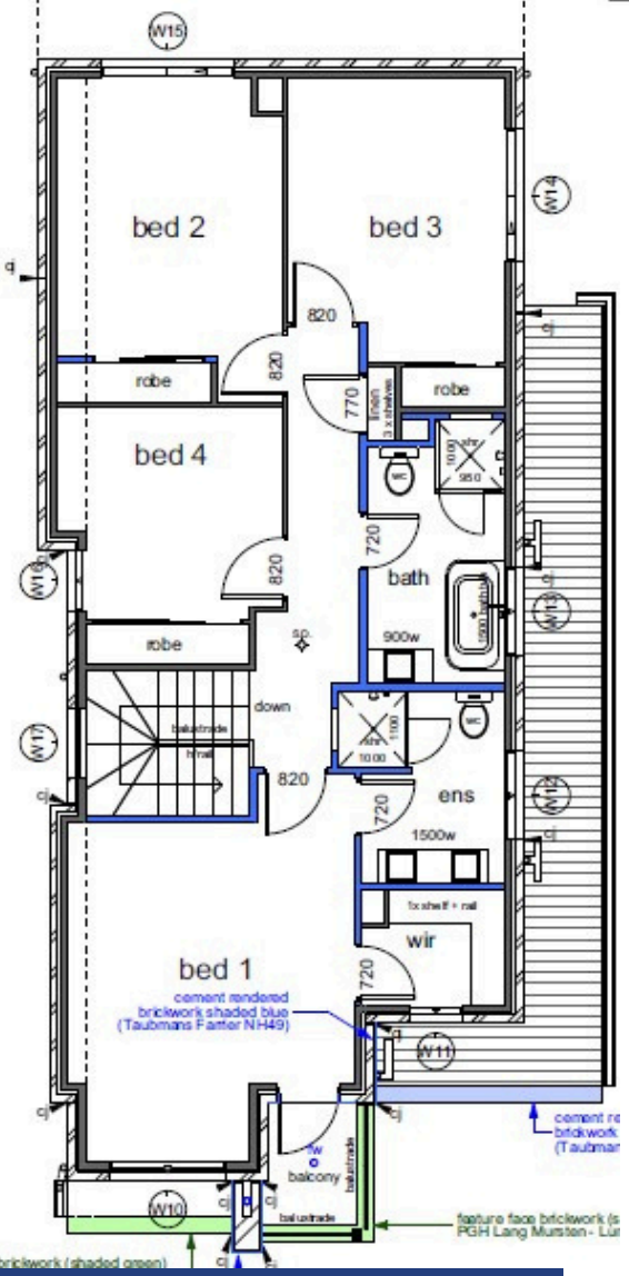
First Floor
