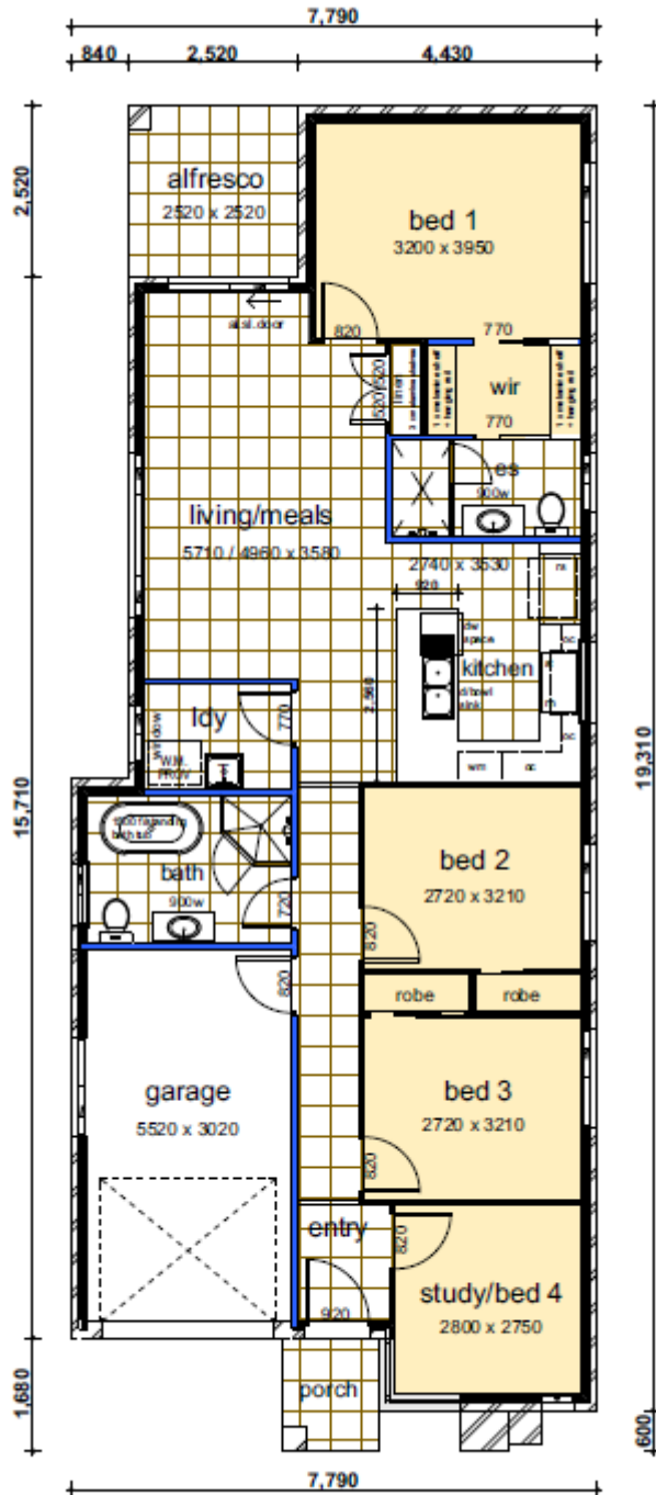
floor plan
