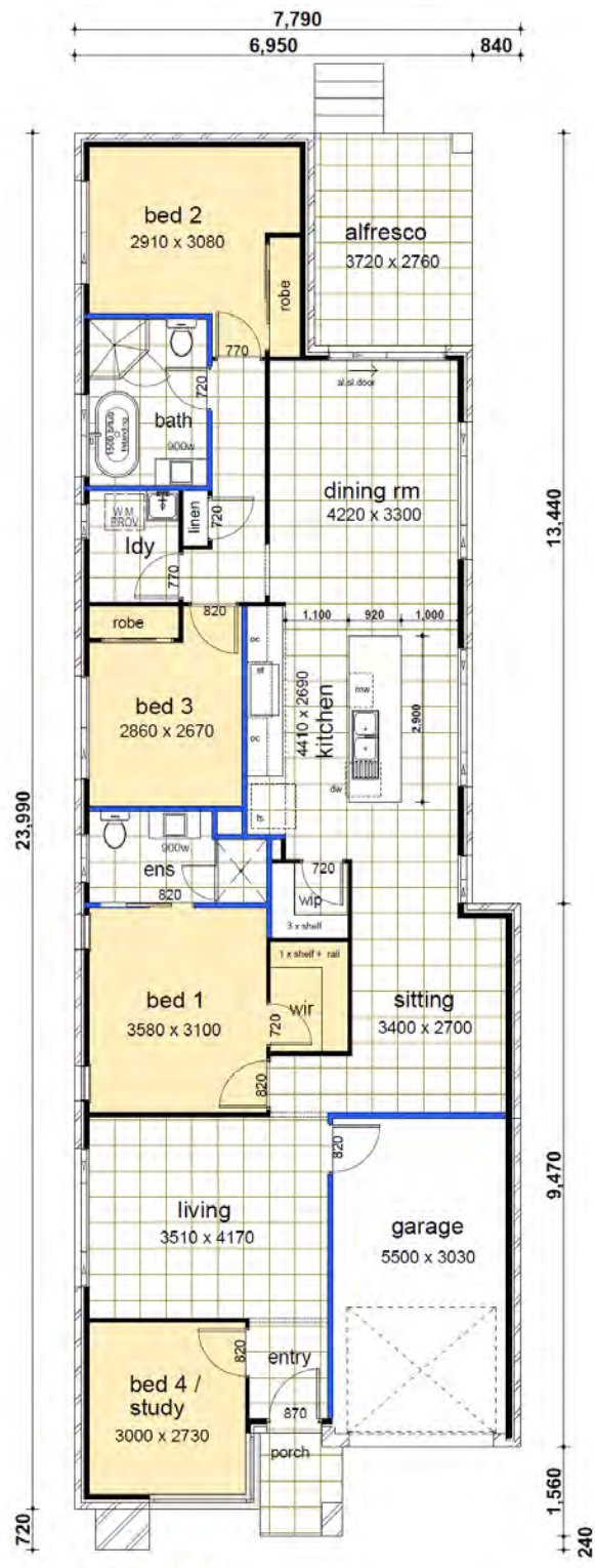
floor plan
