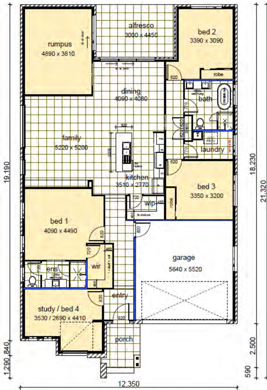
Floor Plan
