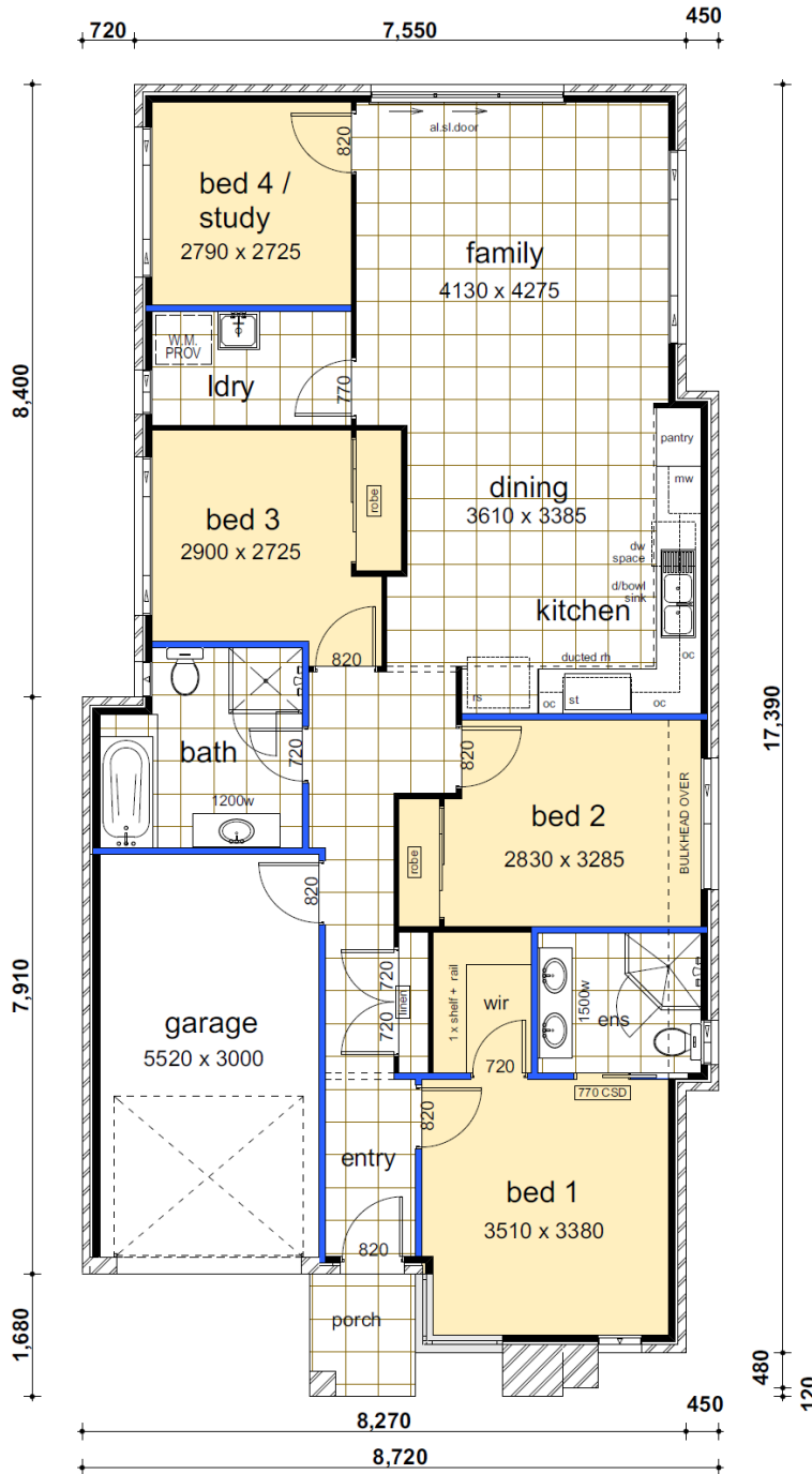
FLOOR PLAN
