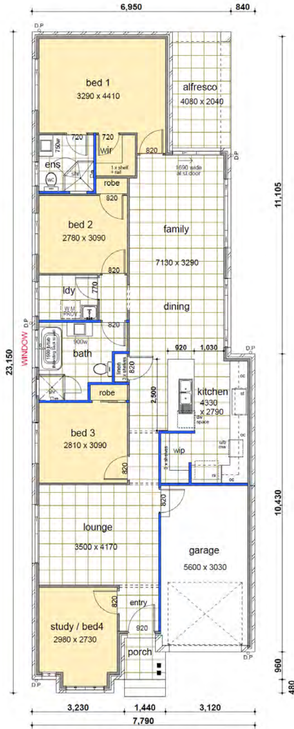
floor plan
