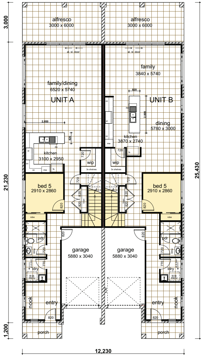
Ground Floor
